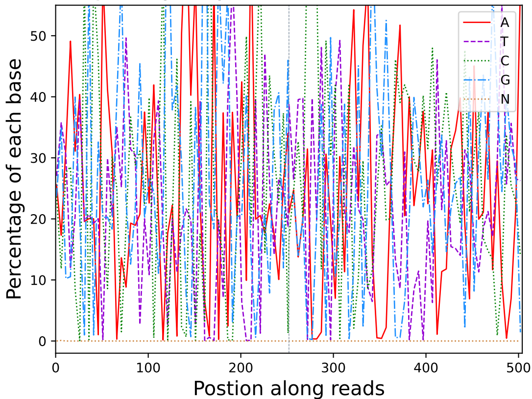
Base percentage along reads (R10320)
